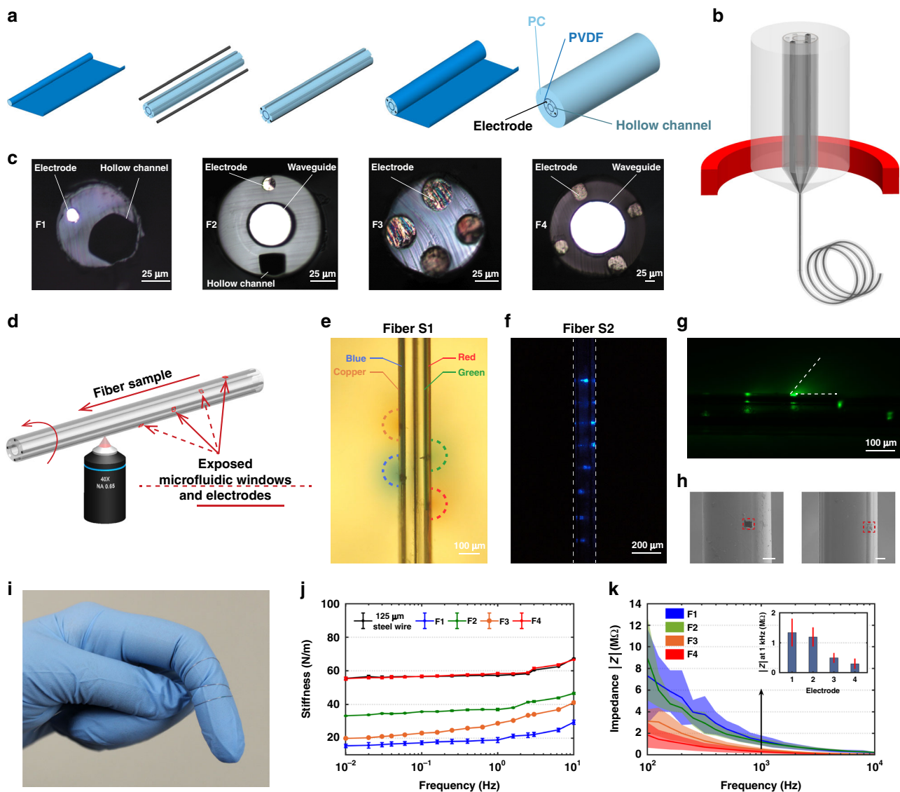
Fig. 1 Depth-dependent multifunctional fiber probe. a A representative multifunctional fiber preform fabrication process (Fiber S1). b A schematic of the Fiber S1 thermal drawing process. c Cross-sectional images of fibers used in this study, electrode (BiSn). d A schematic of femtosecond laser micromachining process on Fiber S1. e-h Validation of the exposed microfluidic, optical excitation, and electrical windows: e four microfluidic windows were created on the four hollow channels of Fiber S1 and four different food colors were injected into the four channels respectively while the fiber was embedded in brain phantom; f an optical image showing the eight optical excitation sites fabricated on the eight waveguides of Fiber S2; g optical microscope image of the exposed Fiber S2 immersed in a drop of fluorescein excited by a 473 nm laser; h SEM images of the exposed microfluidic windows and electrodes (scale bar: 50 \mu\text{m} ). i A photograph of functional fibers. j Bending stiffness measurements of Fiber F1-4. k Impedance measurements of the BiSn electrodes in Fiber F1-4. All error bars and shaded areas in the figure represent the standard deviation.
